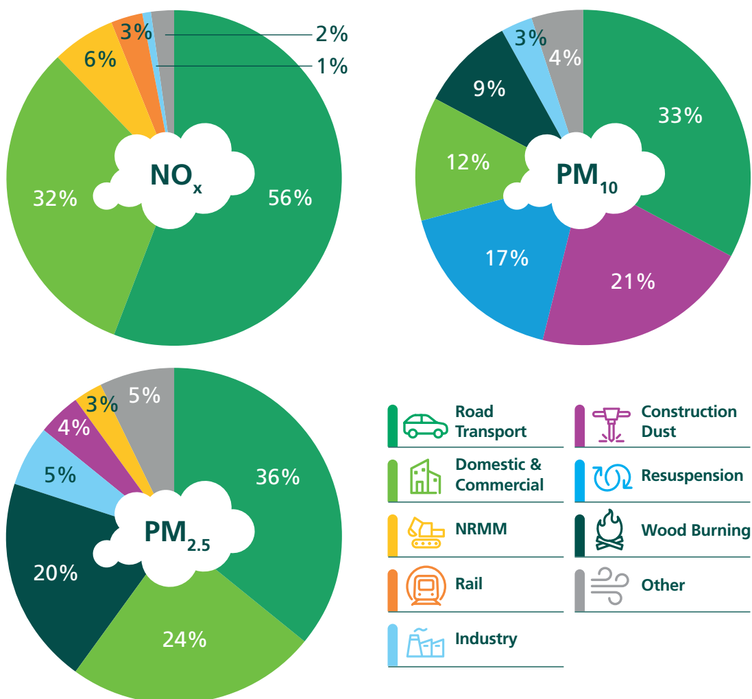
Figure 3.1: Primary emission sources of \text{NO}_x , \text{PM}_{2.5} and \text{PM}_{10} in Ealing (based on LAEI 2019 data) 21
